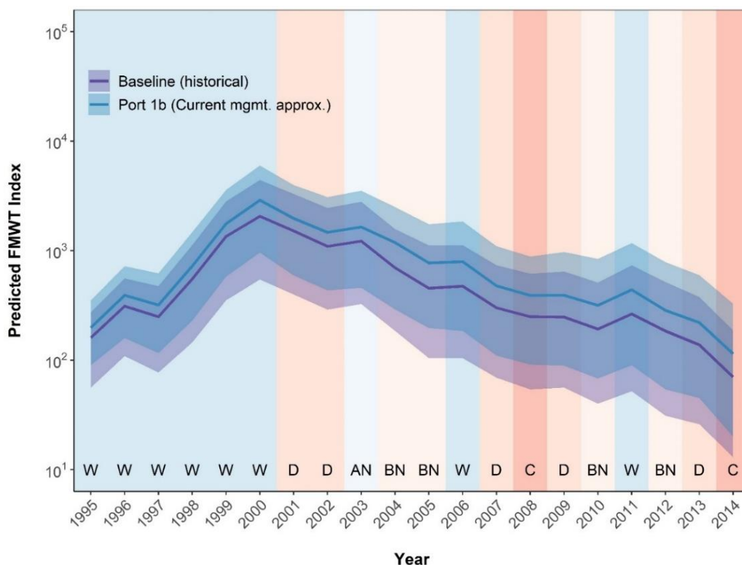
Figure ES-3. Average predicted Delta Smelt FMWT Index across model years (1995-2014) for predicted baseline, historical conditions (purple) and Portfolio 1b (select Delta Smelt management actions in 2019 BiOp/2020 ITP approx.; blue) in the IBMR. The shaded ribbons show the 95% confidence interval (2.5 th and 97.5 th percentiles from the distribution of model predictions) encompassing uncertainty (stochasticity, process variation) in the IBMR. Water year types are indicated by letters at bottom of figure and blue-red bars.
