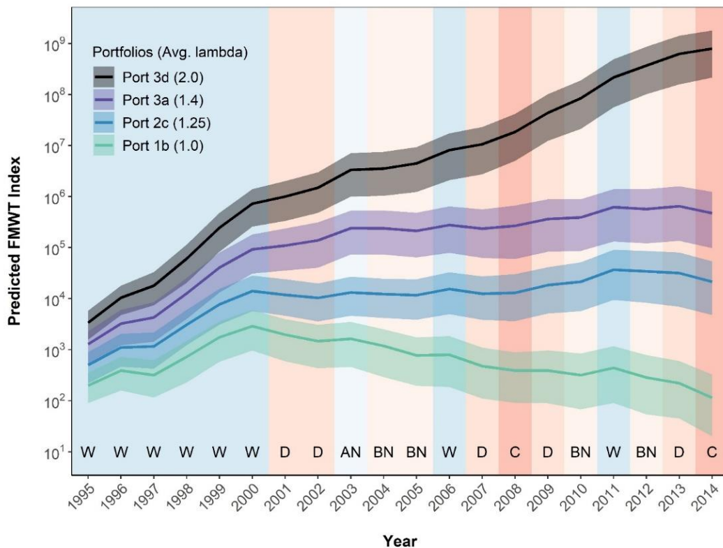
Figure ES-7. Average predicted Delta Smelt FMWT Index across model years (1995-2014) for four portfolios that varied by average growth rate (lambda) in the IBMR. The shaded ribbons show the 95% credible interval encompassing uncertainty (stochasticity, process variation) in the IBMR. Water year types are indicated by letters at bottom of figure and blue-red bars. All portfolios assumed fall X2 \leq 80 km in W and AN years. Portfolio names: 1b – Current management (approximation); 2c – Cache Slough & Suisun Marsh focus, including localized food and turbidity actions; 3a – Self-sustaining / permanent management, including large-scale habitat restoration and contaminant reduction; 3d – Focus on food, including multiple food actions, large-scale habitat restoration, aquatic weed control, and contaminant reduction.
